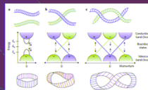
图片来源自Hari Manoharan, Nature Nanotechnology
